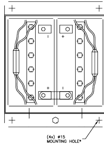
BATTERY BANK PLAN VIEW
